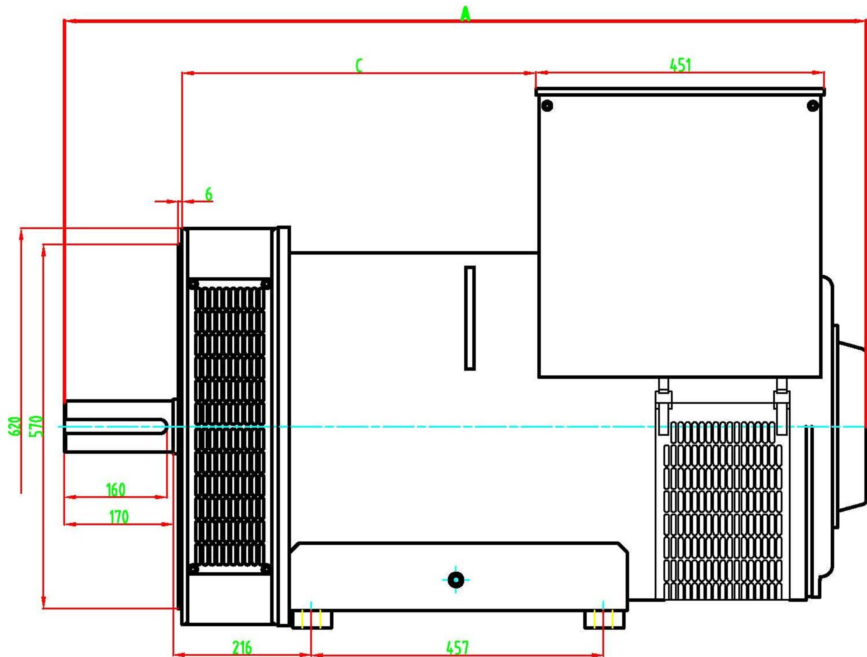
MOUNTING DIMENSIONS/安装尺寸(mm)
