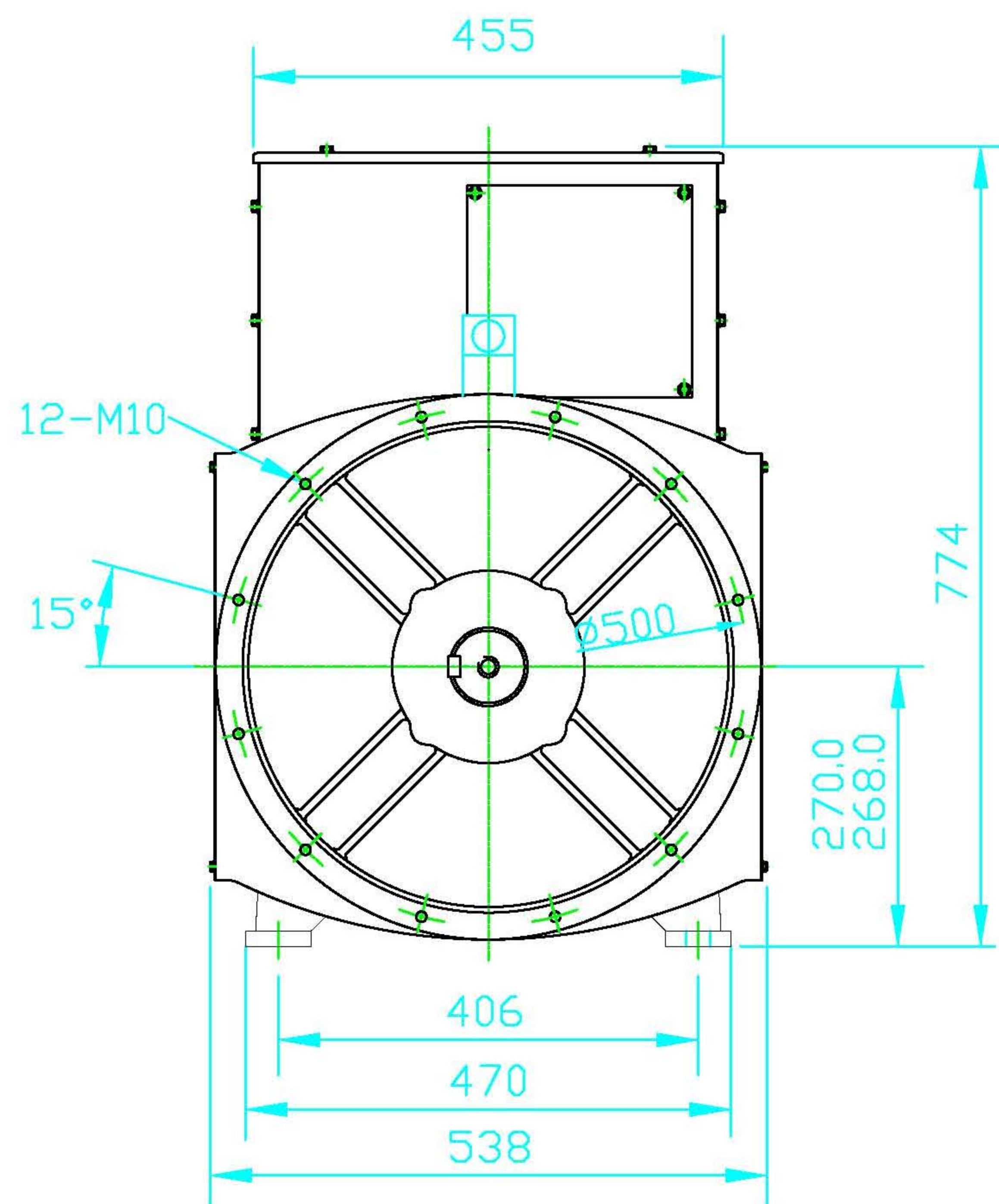
MOUNTING DIMENSIONS(mm)
